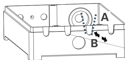
[2:2] Make sockets in enclosures for cabling: LCX and RCX. Use cutting pliers to [A] open the appropriate socket in the enclosure and to [B] trim the socket.
