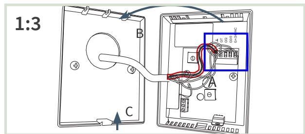
[1:3] [A] In connection with connection: Use bi-conductor hose to shield. Refit the front piece [B] and [C].
